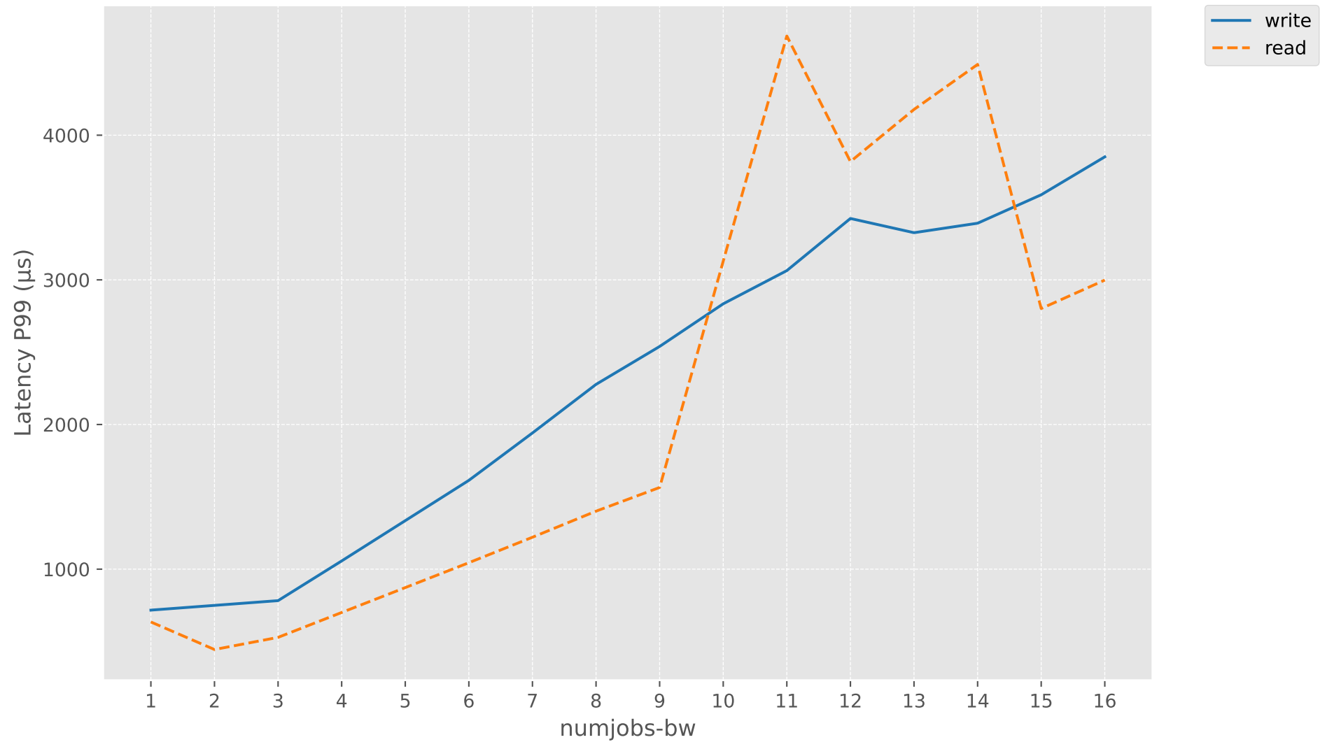
Latency P99 vs numjobs-bw
